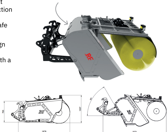
High Tipper Bucket Sweeper SKSM HT
