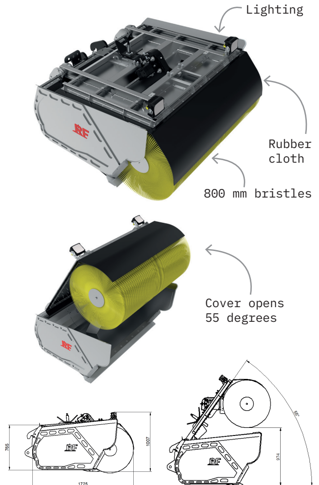
High Tipper Bucket Sweeper SKSM HT
